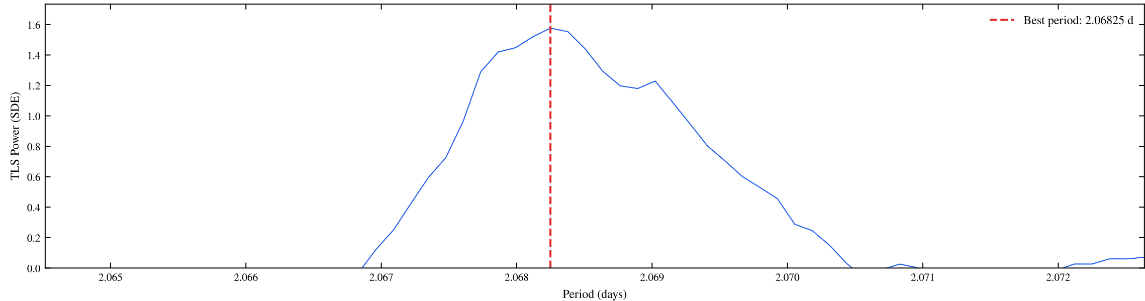
TIC 101230735 | Sectors: 104, 105 | TLS Coarse Periodogram (SDE = 1.58)
