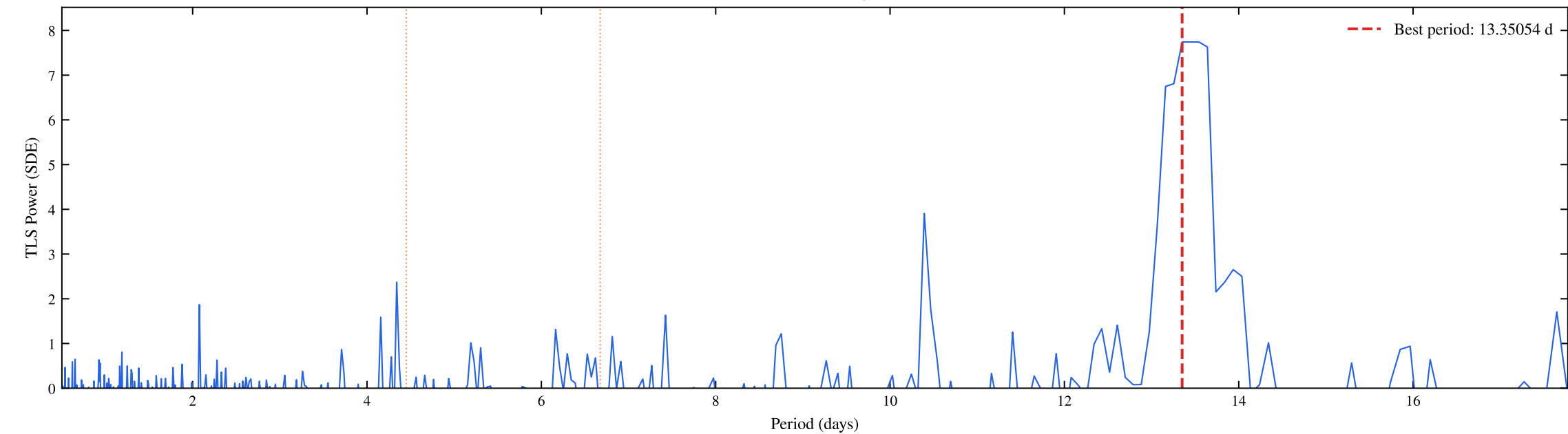
TIC 101230735 | Sectors: 104, 105 | TLS Periodogram (Planet 2 Search) (SDE = 7.74)
