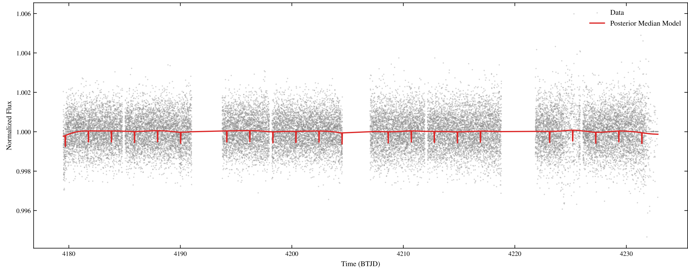
TIC 101230735 | Sectors: 104, 105 | MCMC Posterior Predictive Check
