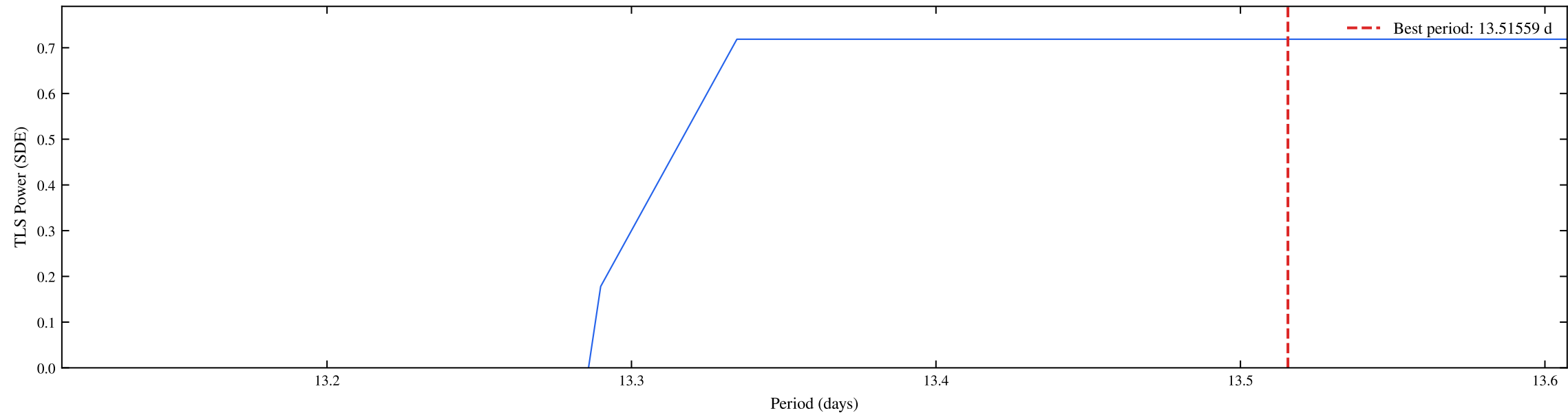
TIC 101230735 | Sectors: 104, 105 | TLS Fine Periodogram (SDE = 0.72)
