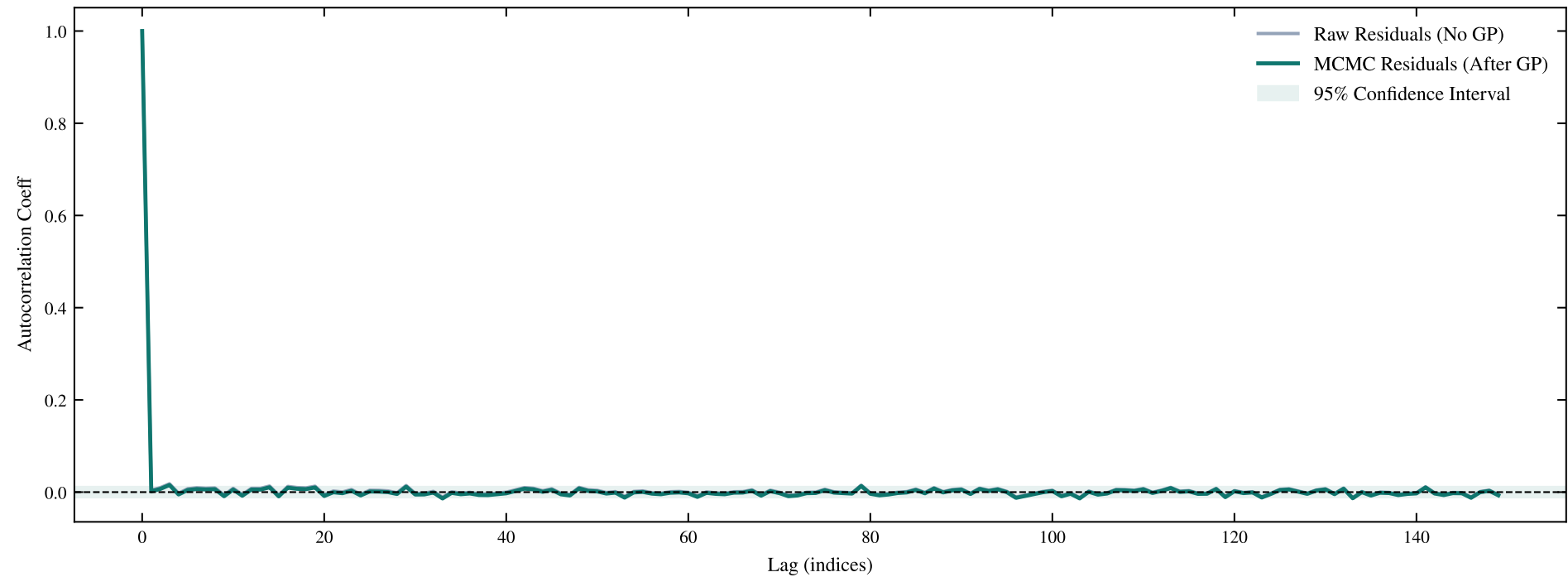
TIC 101230735 | Sectors: 104, 105 | GP Residuals Autocorrelation Function (ACF)
