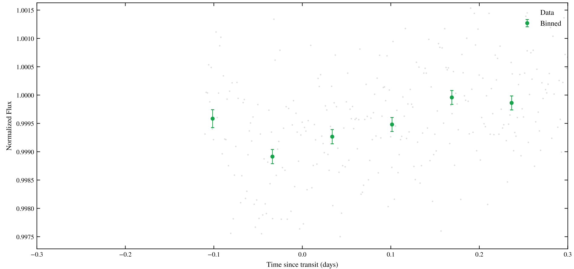
TIC 101230735 | Sectors: 104, 105 | Phase-Folded Transit (P = 13.51559 d)
