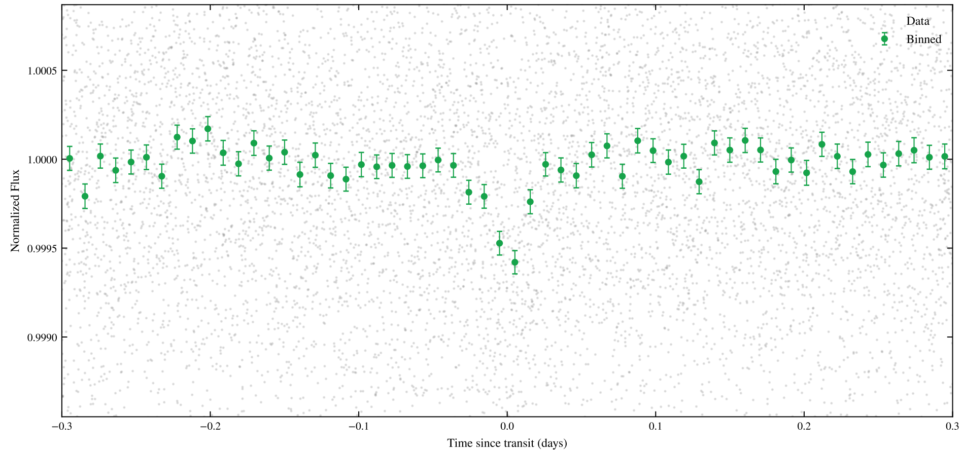
TIC 101230735 | Sectors: 104, 105 | Phase-Folded Transit (P = 2.06825 d)
