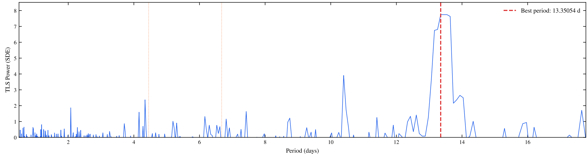
TIC 101230735 | Sectors: 104, 105 | TLS Coarse Periodogram (SDE = 7.74)
